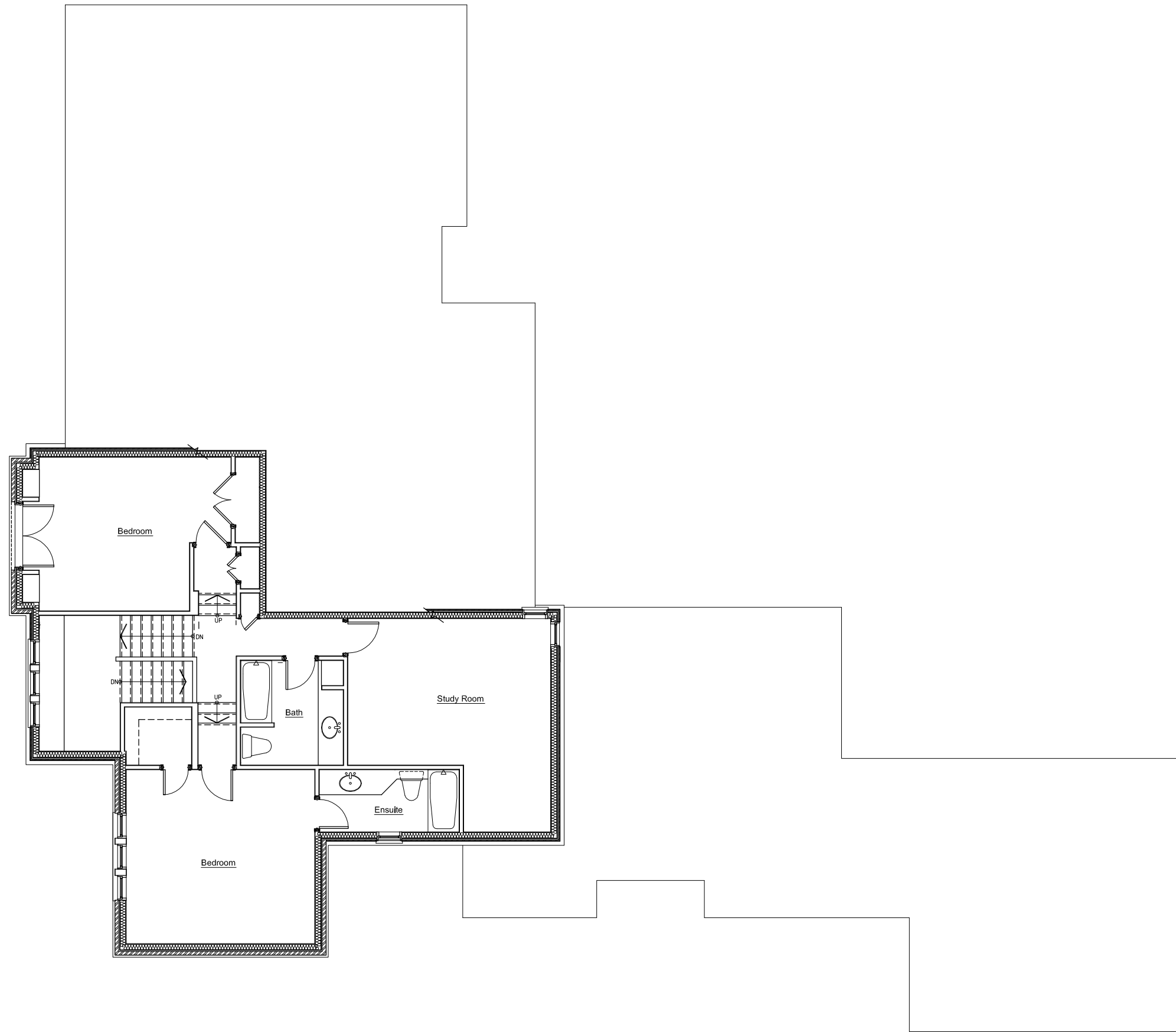
2-Storey Single Family Home 7400 Sq. Ft. Second Floor Plan
